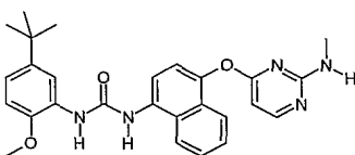
1-(5-tert-Butyl-2-methoxy-phenyl)-3-[4-(2-methylamino-pyrimidin-4-yloxy)-naphthalen-1-yl]-urea;
